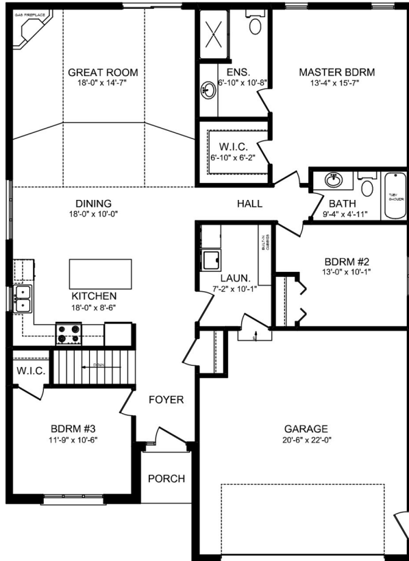
MAIN FLOOR PLAN FINISHED AREA = 1,596 SQ.FT.
