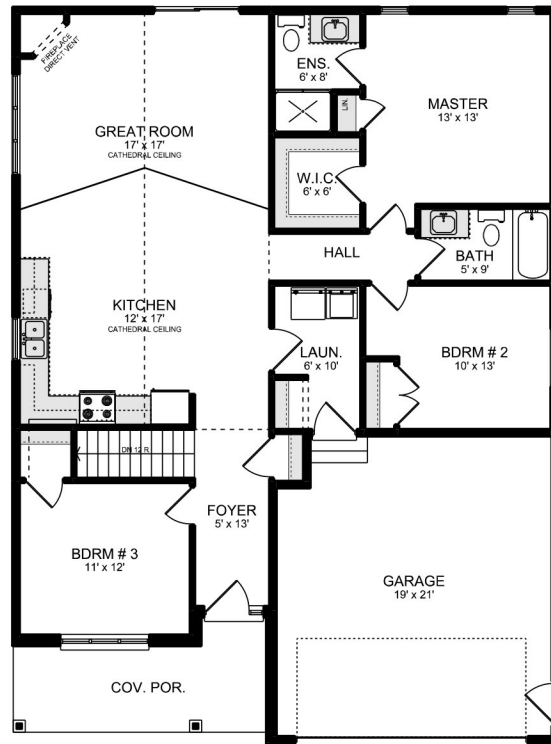
MAIN FLOOR PLAN AREA = 1408 SQ. FT.
