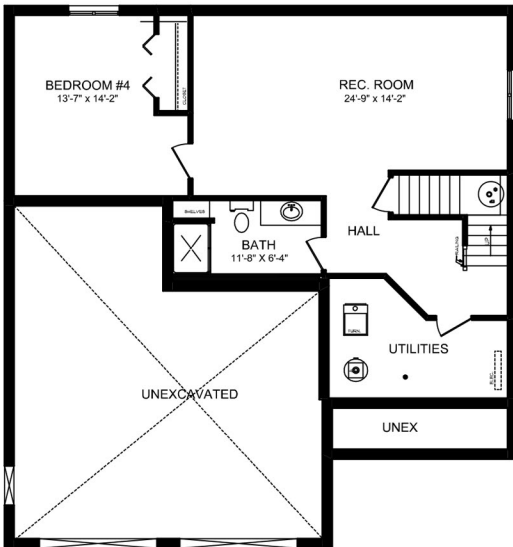
BASEMENT FLOOR PLAN FINISHED AREA = 767 Sq.ft.
