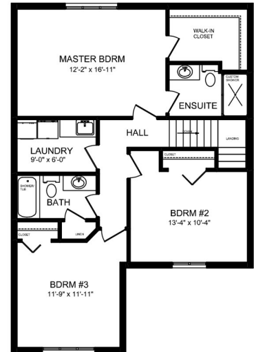
SECOND FLOOR PLAN FINISHED AREA = 950 Sq.ft.
