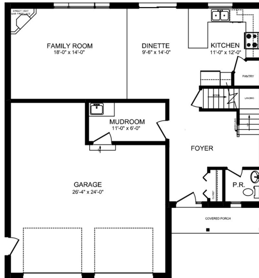
MAIN FLOOR PLAN FINISHED AREA = 938 Sq.ft.
