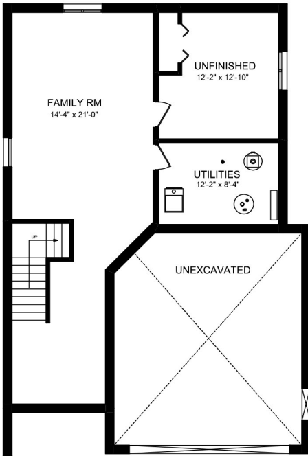
BASEMENT PLAN AREA: 573 SQ.FT.
