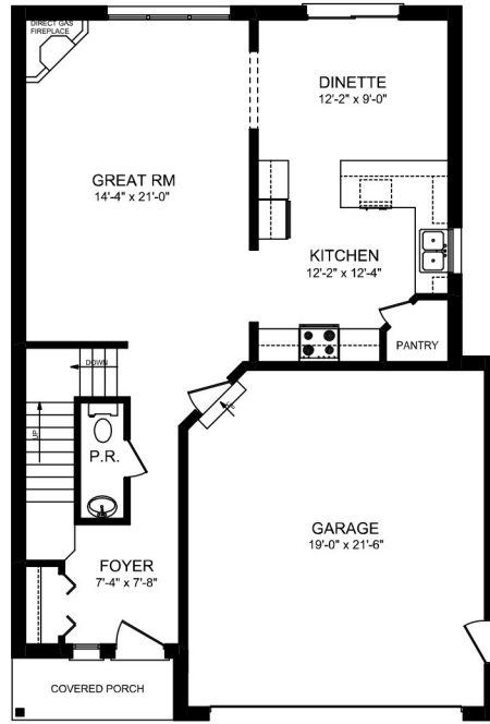
MAIN FLOOR PLAN AREA: 876 SQ.FT.
