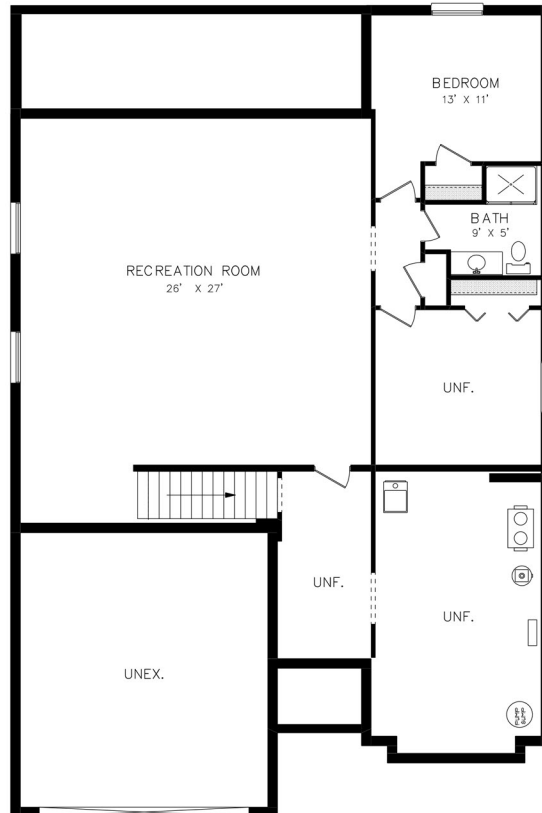
BASEMENT PLAN FINISHED AREA=1037 SQ. FT.
