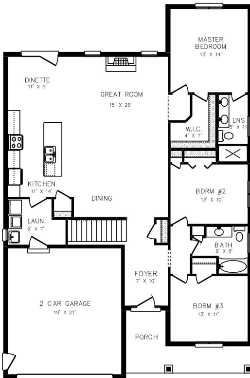
MAIN FLOOR PLAN FINISHED AREA=1824 SQ. FT.
