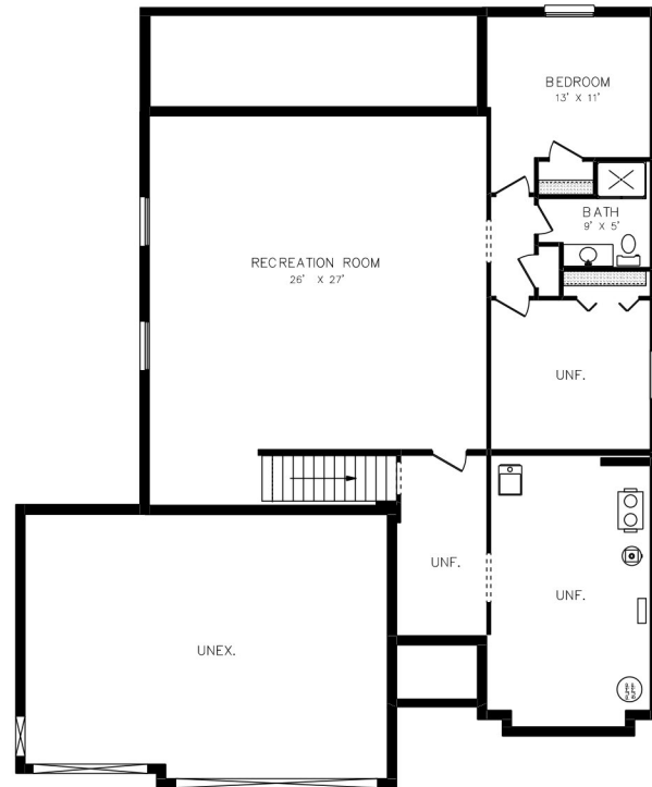
BASEMENT PLAN FINISHED AREA=1037 SQ. FT.
