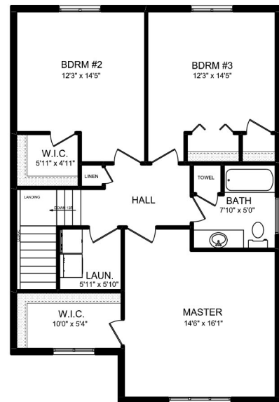
SECOND FLOOR PLAN AREA = 894 Sq.ft.
