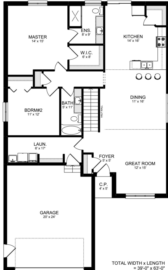
MAIN FLOOR PLAN FINISHED AREA = 1619 Sq.ft.
