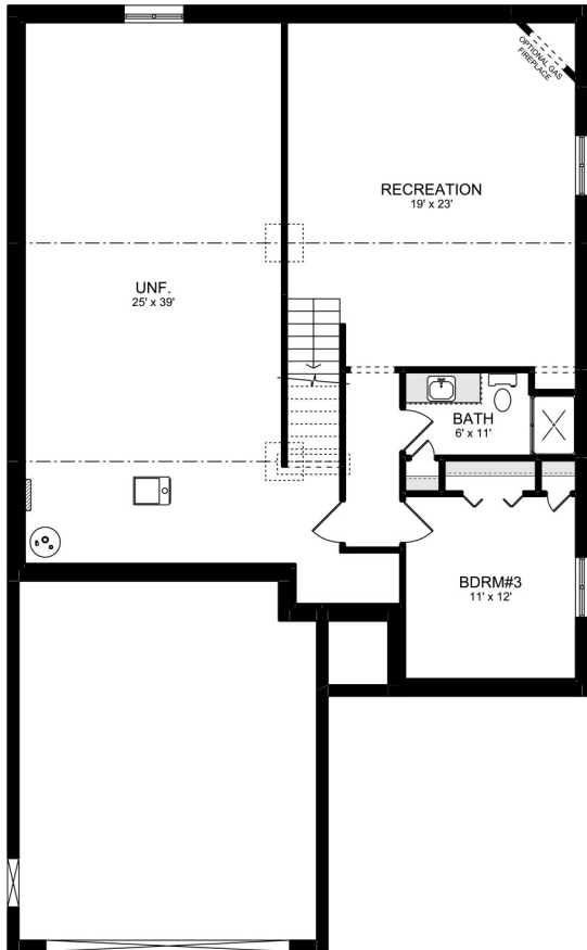
BASEMENT PLAN FINISHED AREA = 700 Sq.ft.
