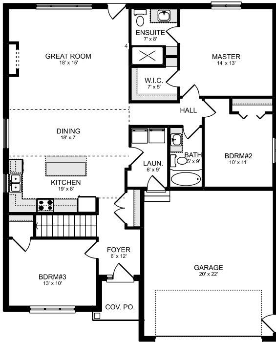
MAIN FLOOR PLAN AREA = 1530 SQ. FT. TOTAL WIDTH X LENGTH = 51'-0" X 41'-6"
