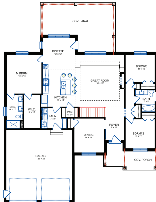
MAIN FLOOR PLAN AREA: 1862.2 Sq. Ft. TOTAL WIDTH x LENGTH = 56'-8" x 77'-10"
