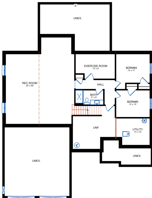
BASEMENT PLAN AREA: 1101.1 Sq. Ft. TOTAL WIDTH x LENGTH = 56'-8" x 77'-10"
